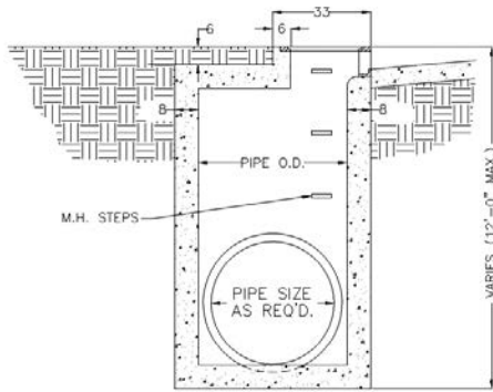
SECTION VIEW
